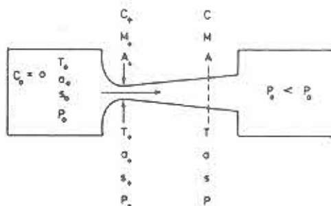
Fig. 5.6 Flow from a reservoir through a convergent-divergent nozzle
