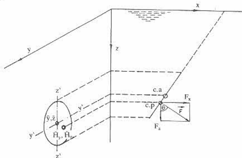
Fig. 2.12 Flat plate submerged in a static incompressible fluid
