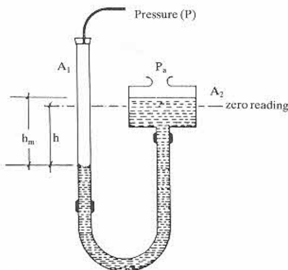
Fig. 2.8 Well-type manometer
