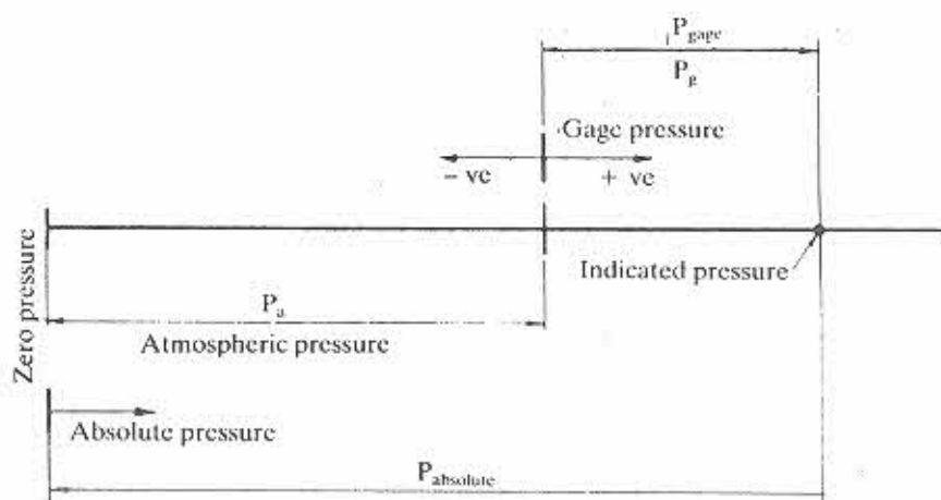
Fig. 2.4 Absolute and gage pressures
