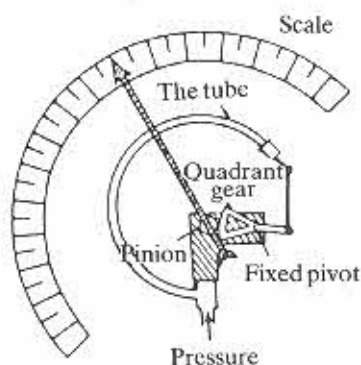
Fig. 2.10 Bourdon gauge
