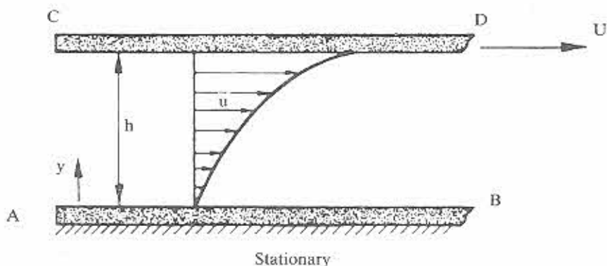
Fig. 1.1 Fluid motion between two parallel flat plates
