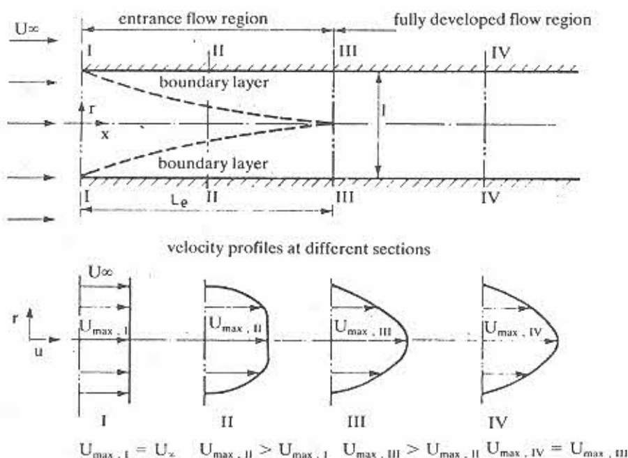
Fig. 4.5 Entrance and fully developed flow regions in a conduit
